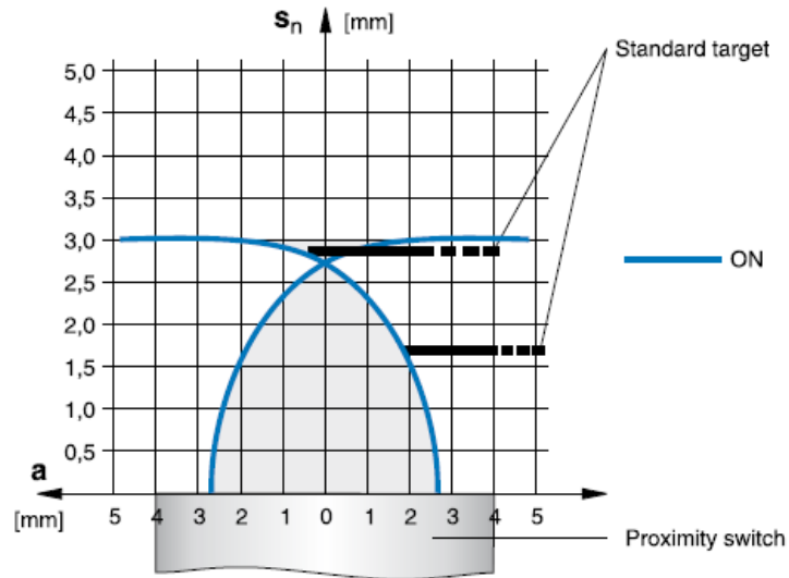
Response diagram:
